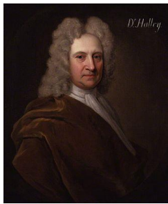
Edmond Halley
